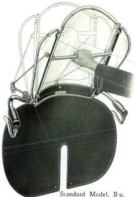
Standard Model, B 9.
